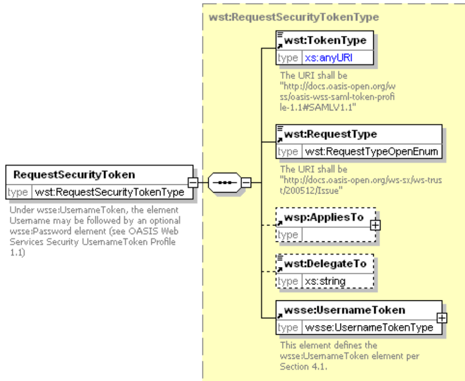
Figure 14 RequestSecurityToken schema
