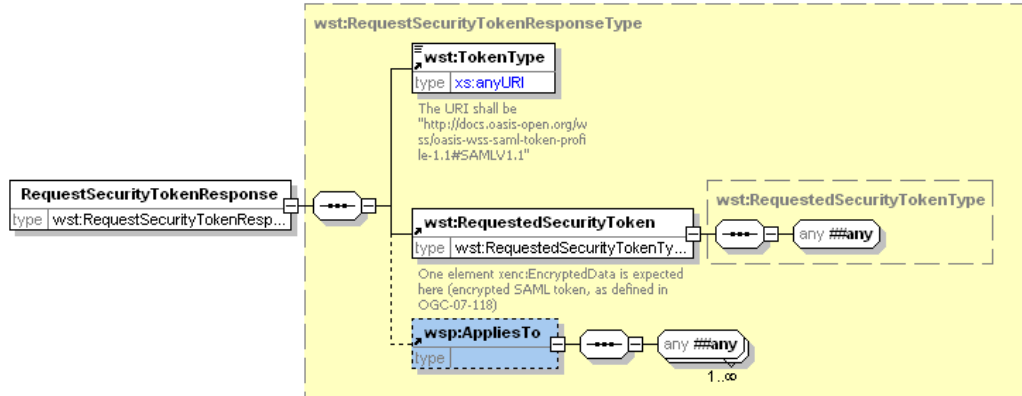
Figure 15 RequestSecurityTokenResponse schema
