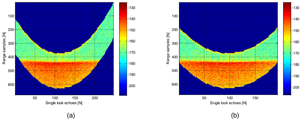
Fig.2 Surface Sample Stack power in dB: before Surface Sample Stack Weighting (a) and after Surface Sample Stack Weighting (b).
