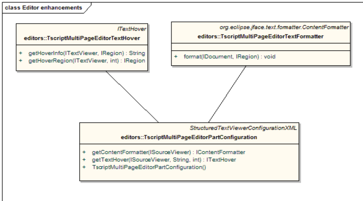
Figure 12 Text Hover class for Toolbox Editor
