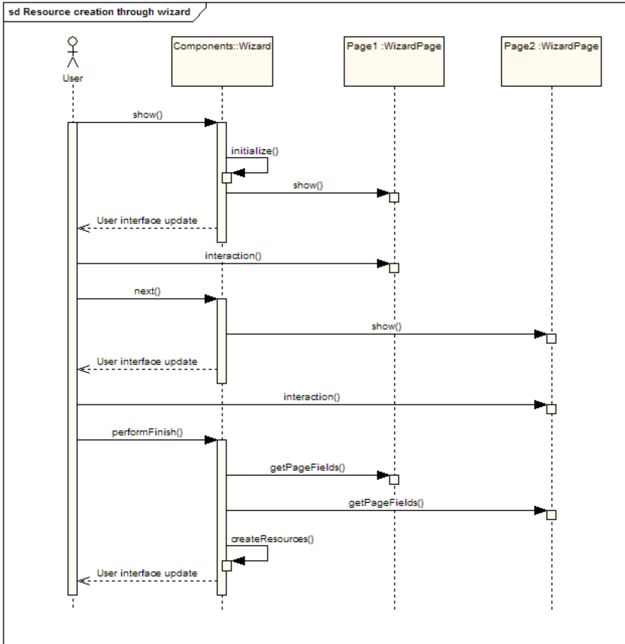
Figure 16 Sequence diagram showing interactions between user and wizards
