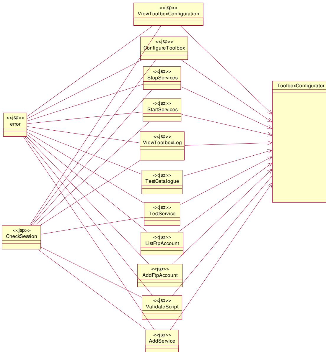
Figure 7 Toolbox Configurator and jsp relationships
