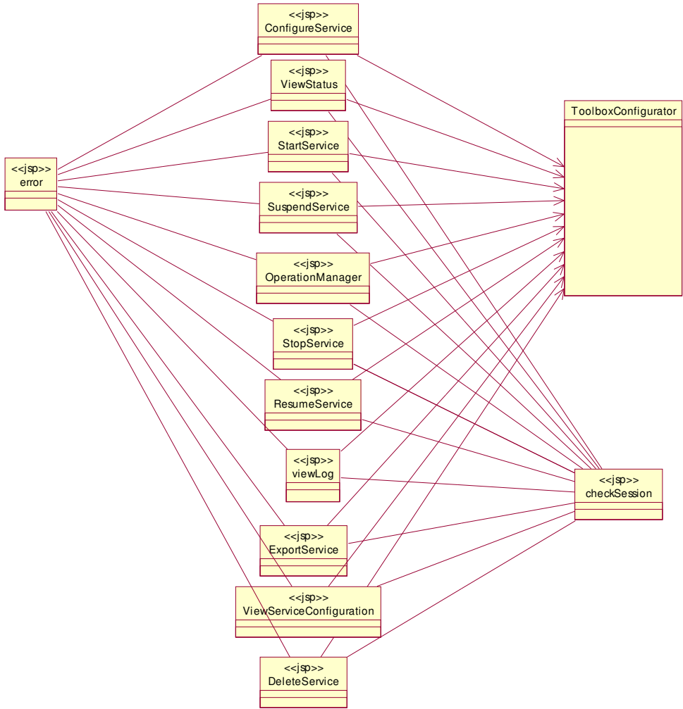
Figure 8 Check session and jsps relationships
