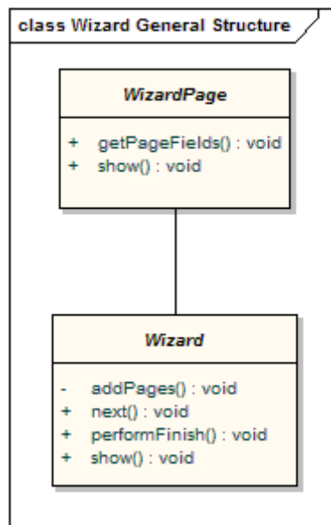
Figure 9 Wizard classes structure
