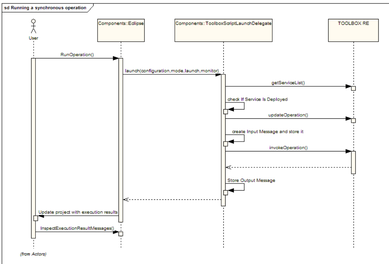
Figure 17 Sequence diagram of a synchronous operation execution
