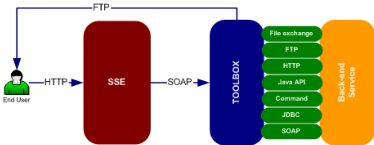
Figure 1 The SSE - TOOLBOX - Back-end service interaction
