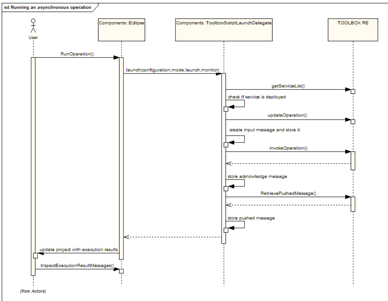
Figure 18 Sequence diagram of an asynchronous operation execution
