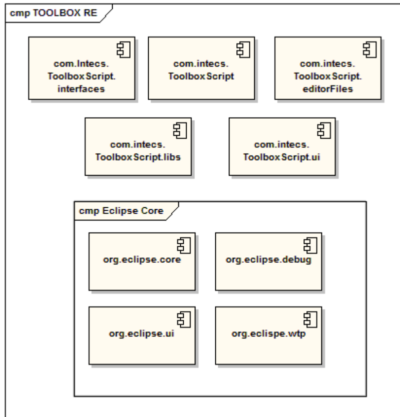
Figure 6 High level TOOLBOX DE plug-ins structure
