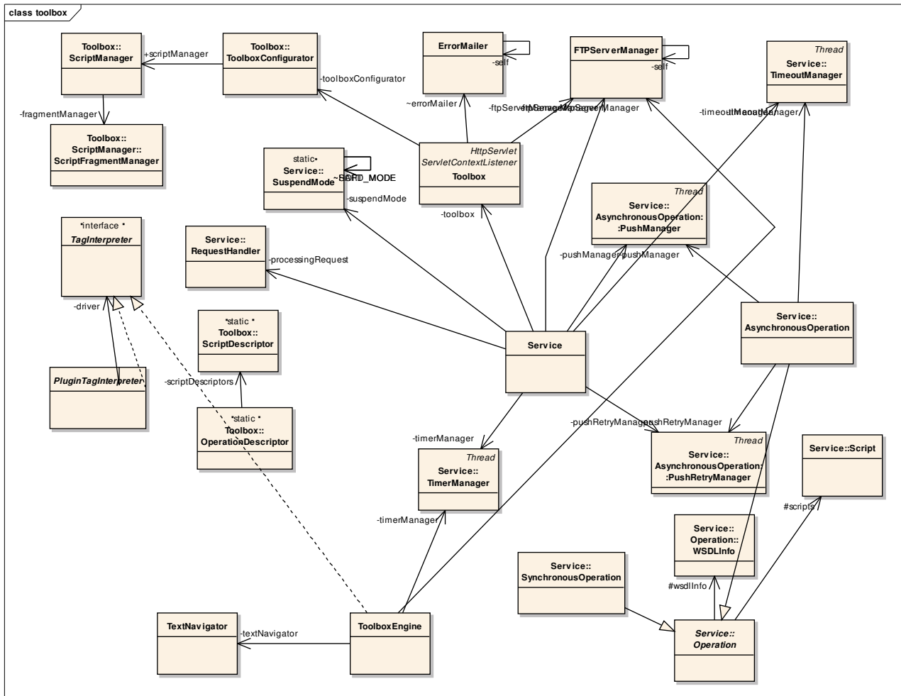
Figure 13 TOOLBOX RE internal dependencies and interfaces.
