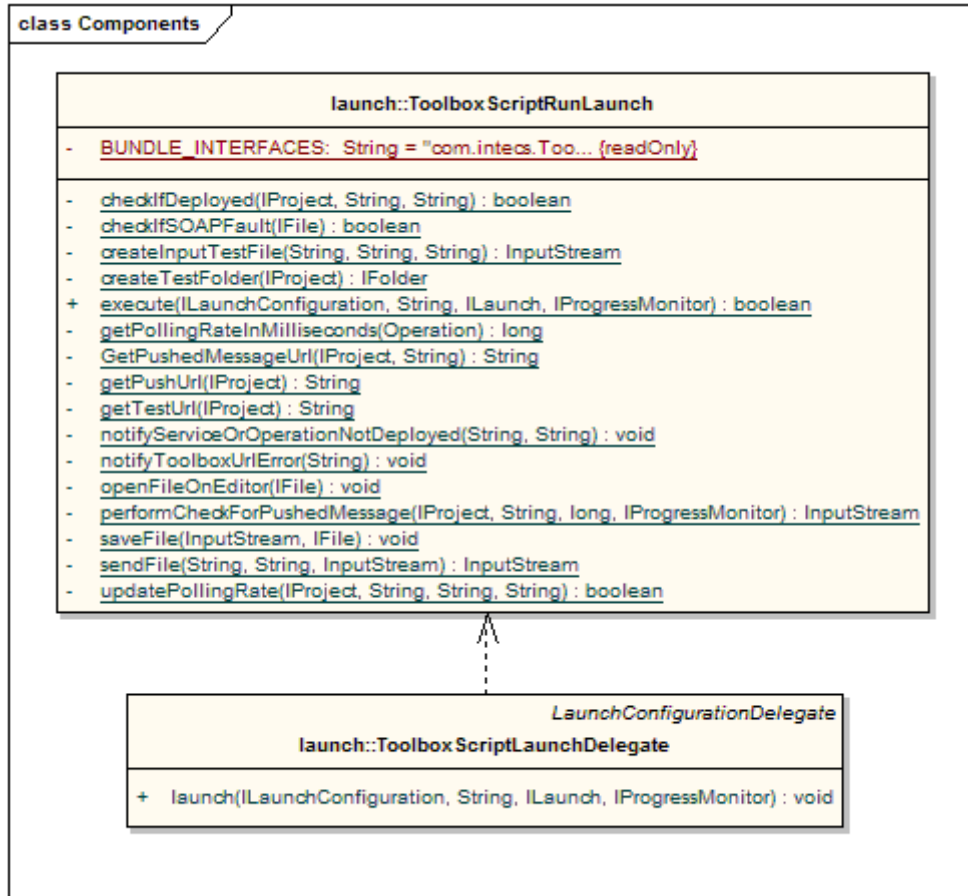
Figure 10 LaunchDelegate class structure diagram
