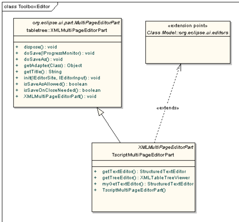
Figure 11 Toolbox Editor class diagram
