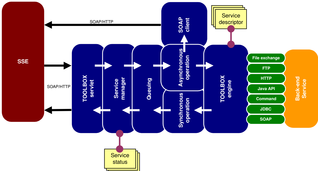
Figure 5 TOOLBOX high level decomposition
