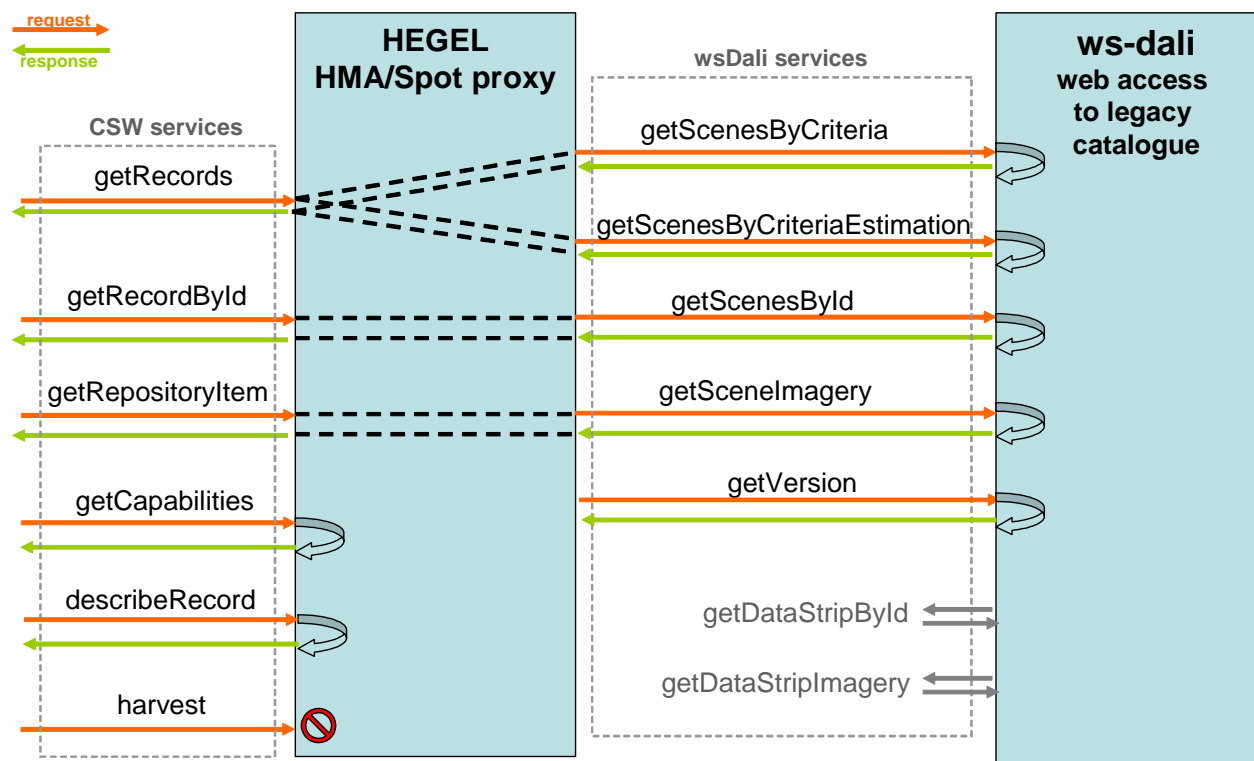
Figure 1 : Mapping of services between HMA and ws-dali
