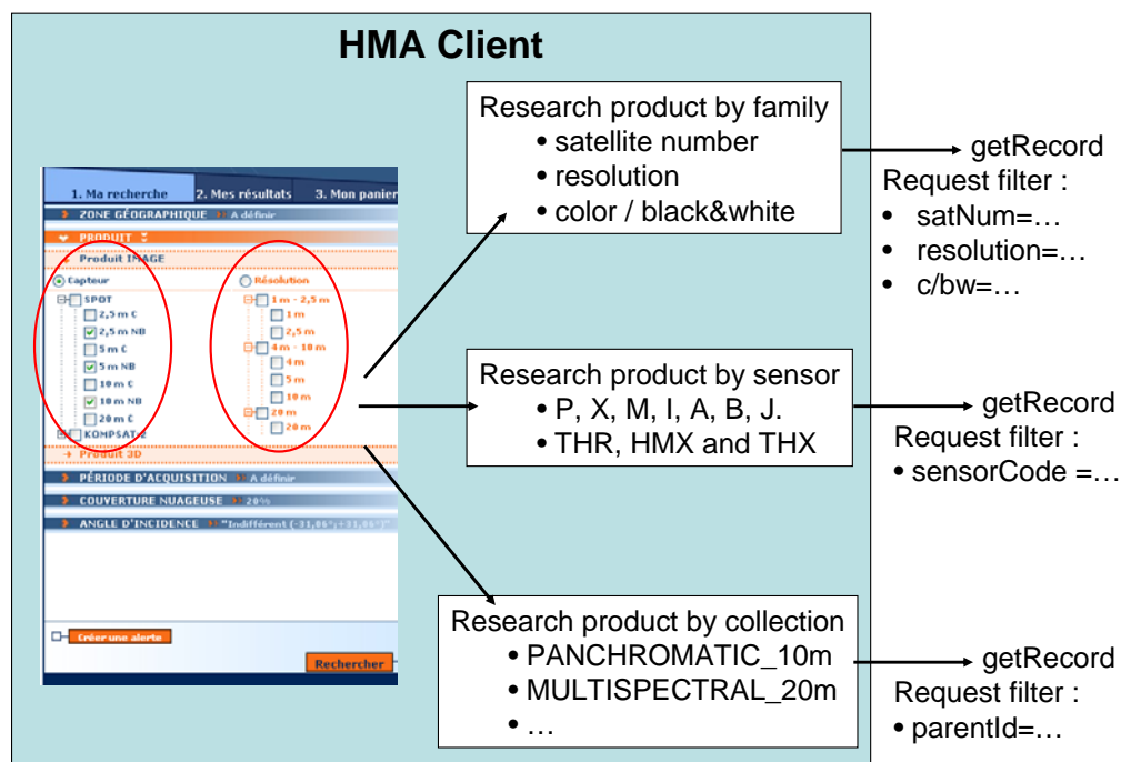
Figure 2 : Different types of requests for HMA client
