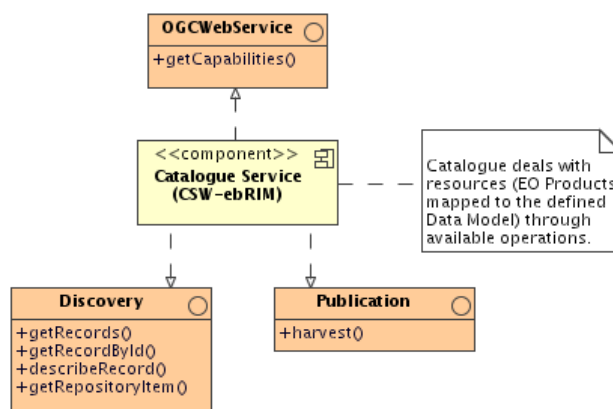
Figure 16: Service Interface (CSW-ebRIM)
