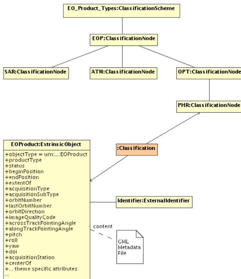
Figure 11: EO Product classified
