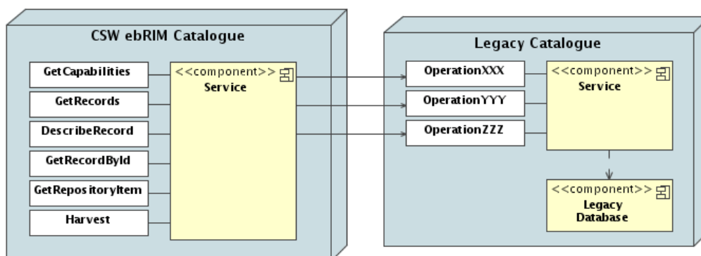
Figure 19: Front-End Architecture
