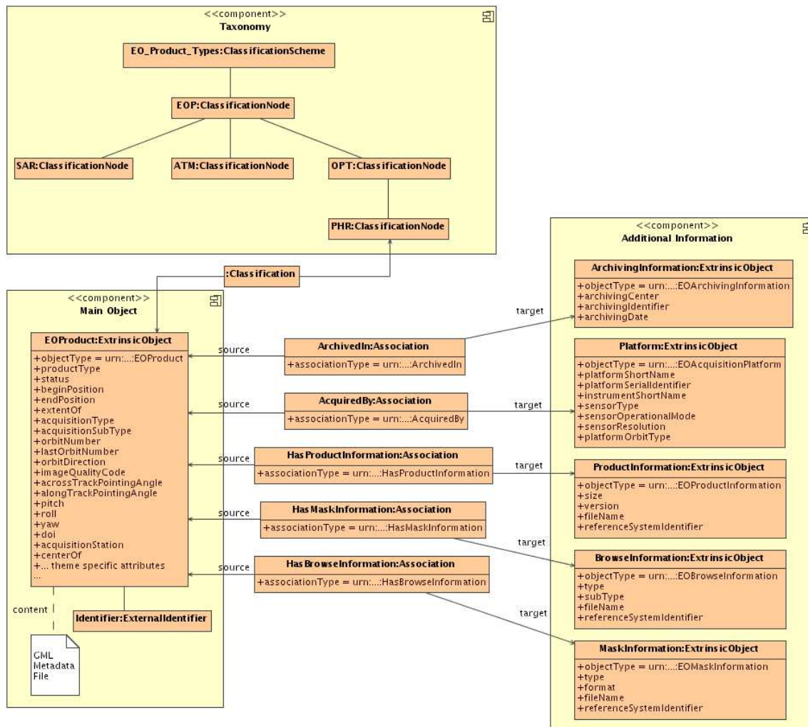
Figure 14: Complete EO Products Data Model
