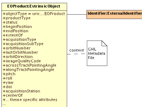
Figure 9: EO Products instance
