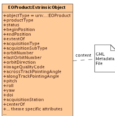
Figure 8: EO Products instance
