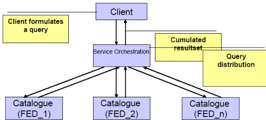
Figure 17: Implementing distributed search
