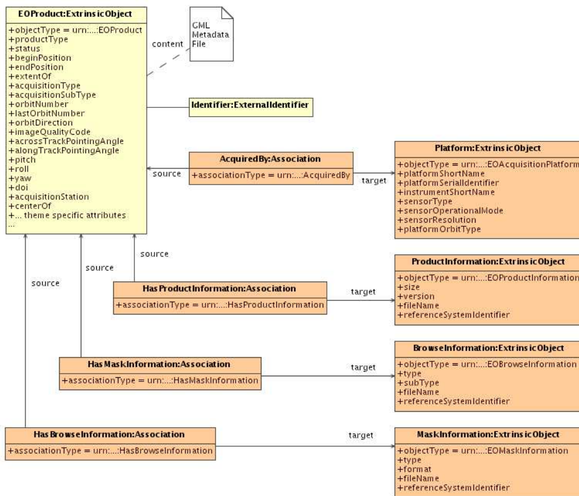
Figure 12: EO Products additional information
