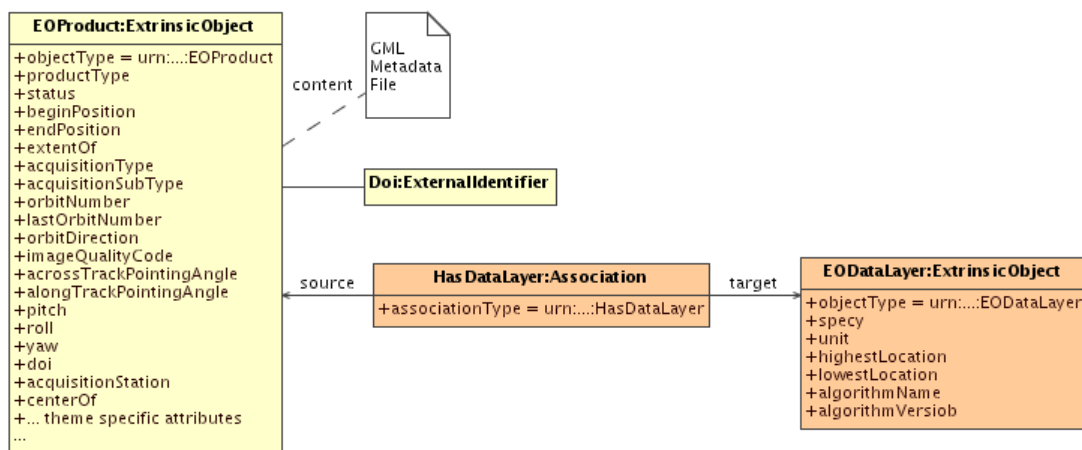
Figure 15: EO Data Layers associated to EO Products
