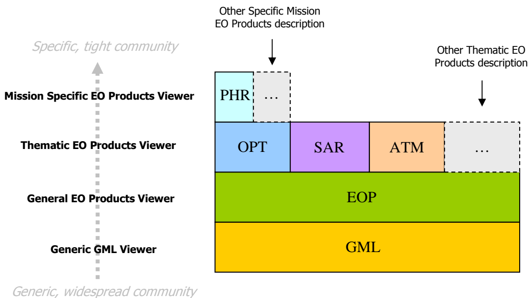
Figure 5 : A layered view of GML EO Products data.
