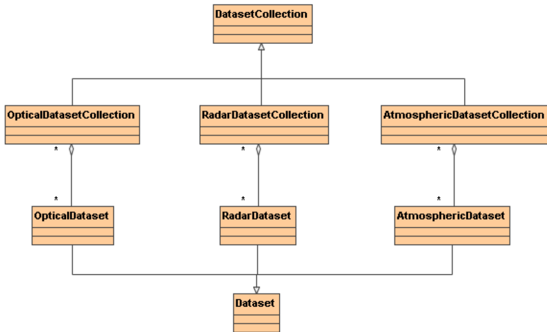
Figure 4: Relationship between EO dataset collections and datasets
