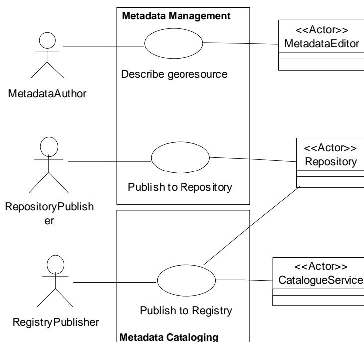
Figure 2: Publish metadata
