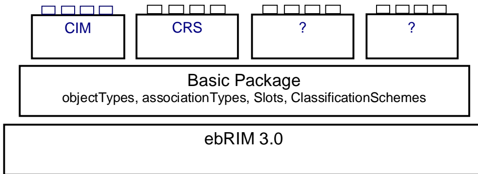
Figure 3 Extension packages 1
