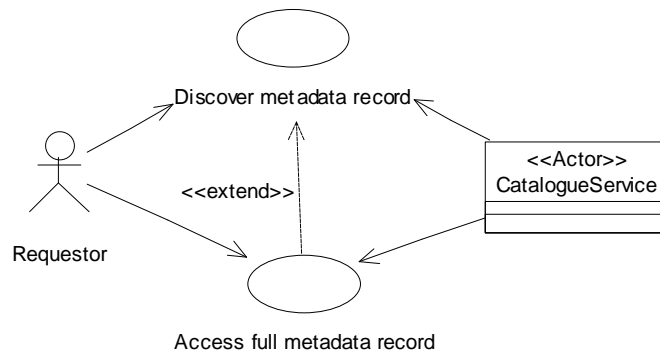
Figure 3: Discover metadata
