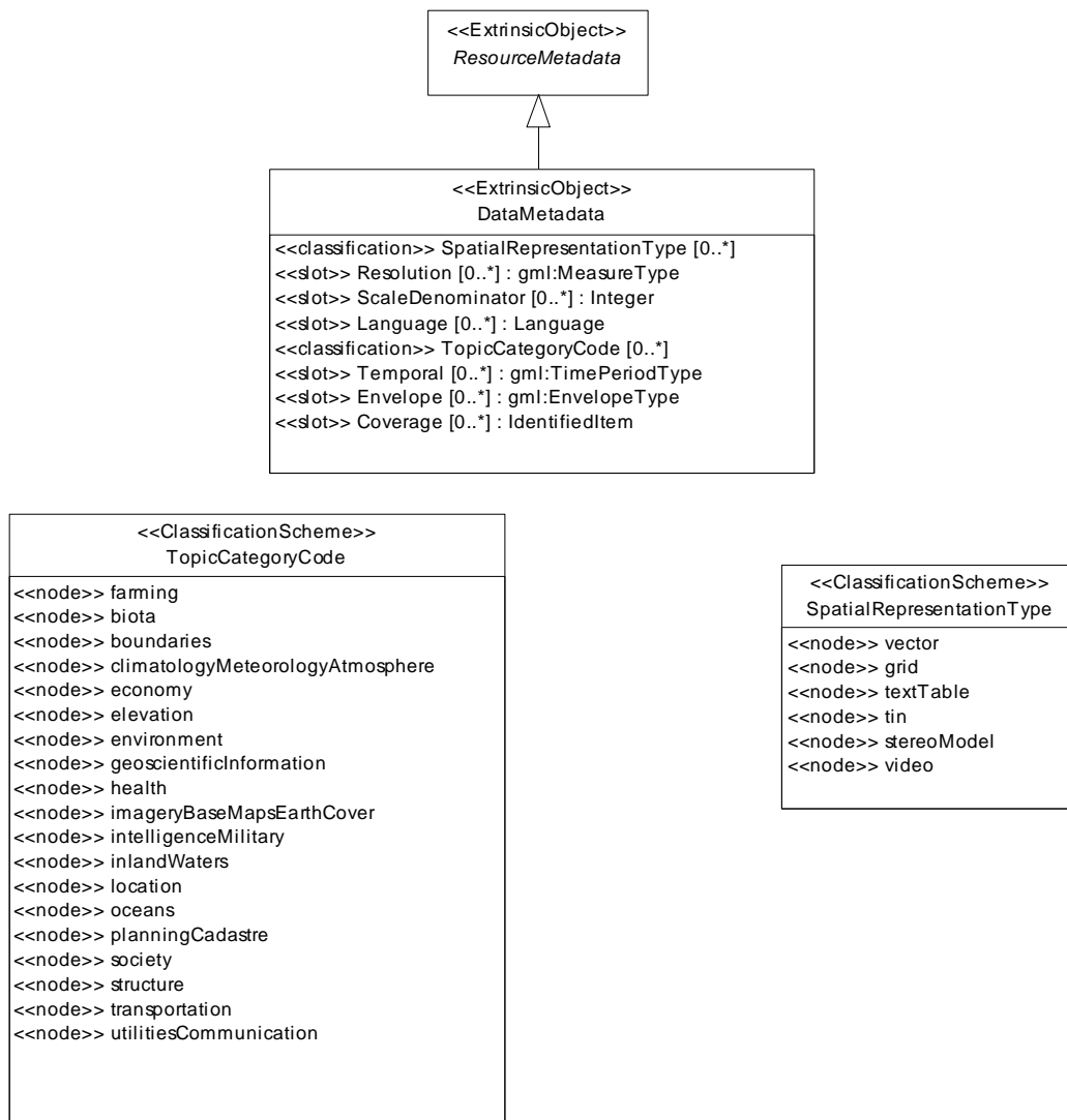
Figure 7 6 Data Metadata
