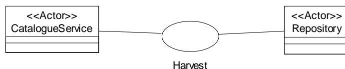
Figure 4: Harvest metadata
