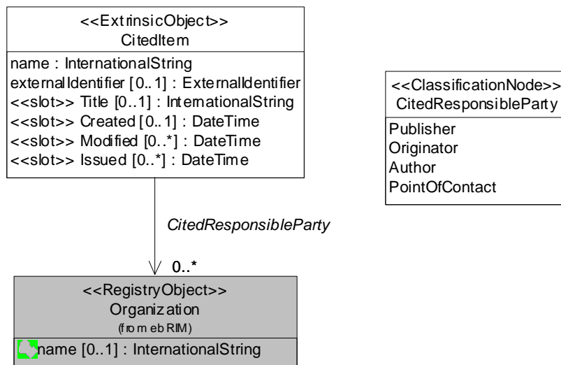
Figure 12 ó Citation
